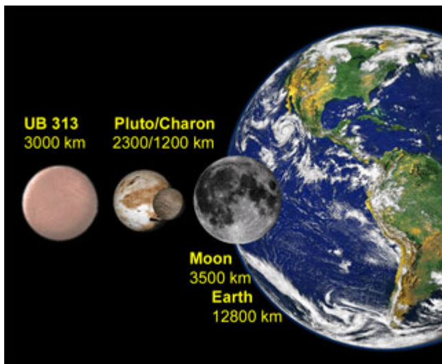
Fig. 1: The diameter of 2003 UB313 compared with that of the Pluto, Charon, Earth, and the Moon.
