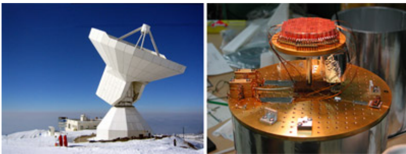
Fig. 2: To detect the very faint millimeter wavelength emission from UB313, the Bonn group used the IRAM 30-m telescope on Pico Veleta in the south of Spain, and the very sensitive heat sensor MAMBO-2, which was developed and built at the MPIfR in Bonn by the group of Dr. Ernst Kreysa. The Institute for Radio Astronomy at Millimeter wavelengths (IRAM) is supported jointly by the German Max Planck Society, the French Centre National de Recherche Scientifique (CNRS) and the Spanish Instituto Geográfico Nacional.
